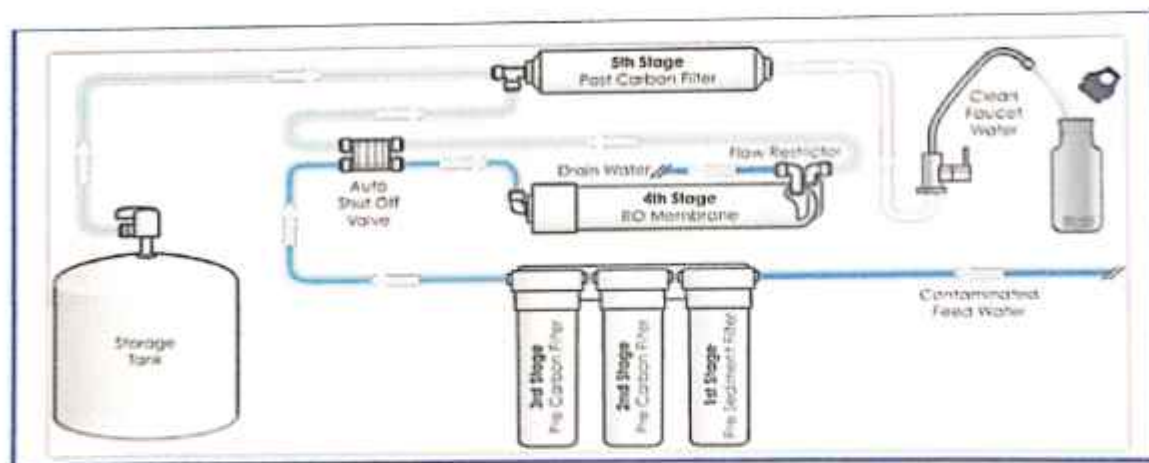
Water purification process outline
